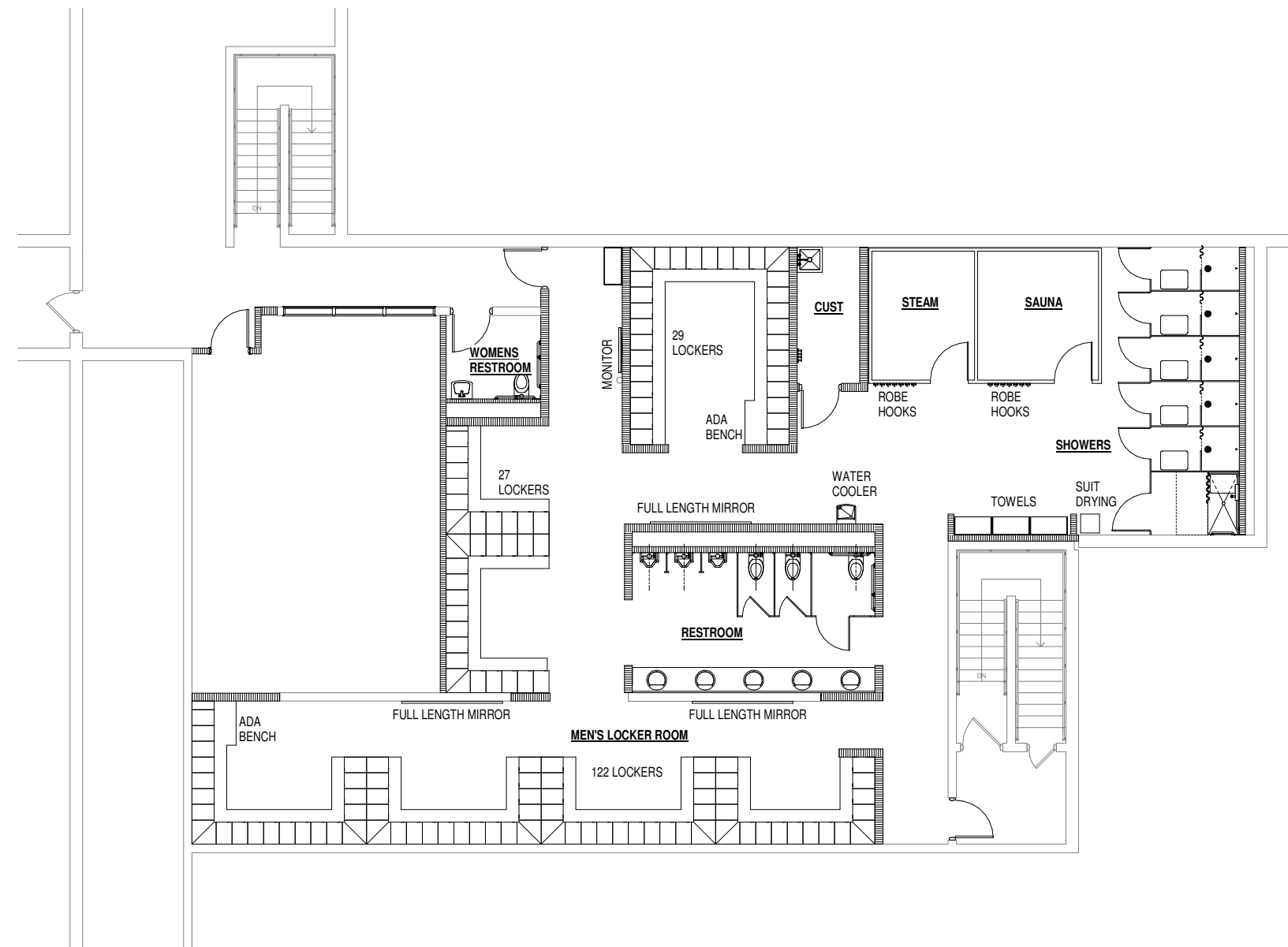
SECOND FLOOR LOCKER ROOM EQUIPMENT PLAN
