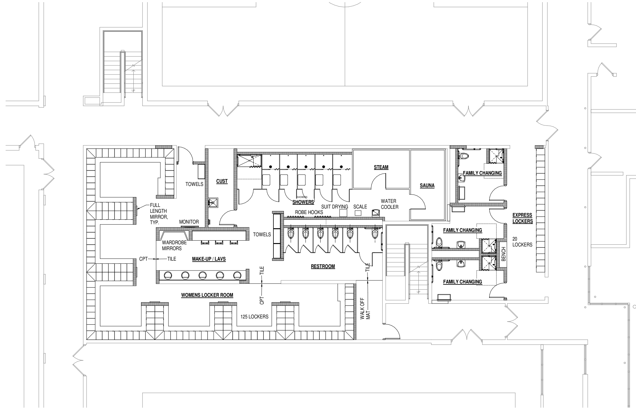
FIRST FLOOR LOCKER ROOM EQUIPMENT PLAN
